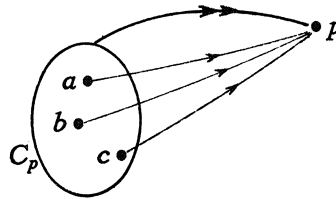
Figure 1. The collection C_p is represented by the set p . The single arrows denote the \in -relation, the double arrow visualizes representation.
