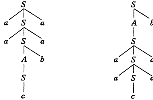
Figure 3. Derivation trees of aacbaa and aacaab .
